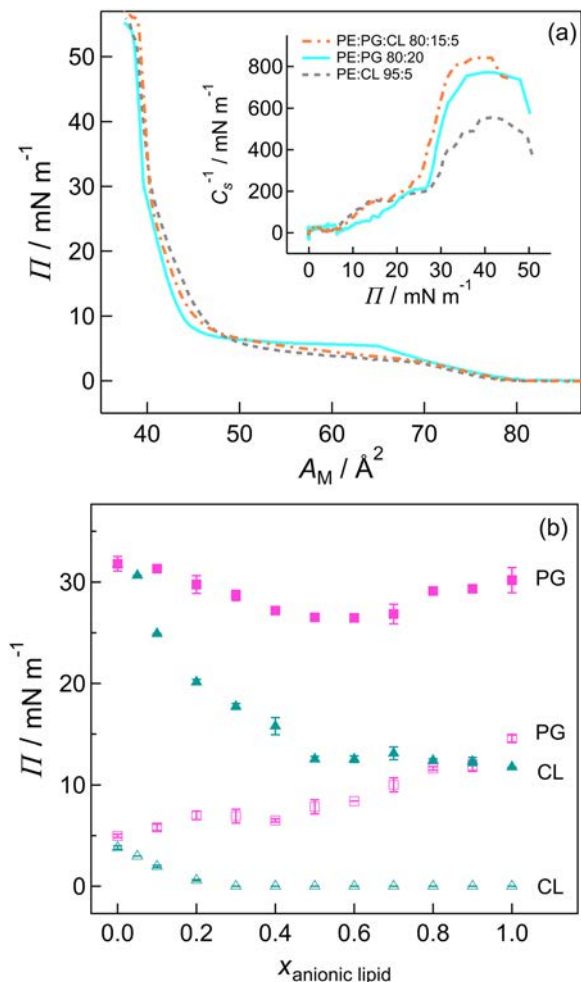
Fig. 1 (a) Surface pressure-area isotherms of PE:PG 80:20 (solid cyan line), PE:CL 95:5 (dashed grey line) and PE:PG:CL 80:15:5 (dash-dotted orange line). Barrier speed 25 \text{ cm}^2 \text{ min}^{-1} , temperature 19.5 \text{ }^\circ\text{C} . The inset shows the corresponding compressibility moduli. (b) L_c -S (filled shapes) and L_e - L_c (open shapes) phase transition pressures vs. mol fraction anionic lipid. Pink squares PG, teal triangles CL.
