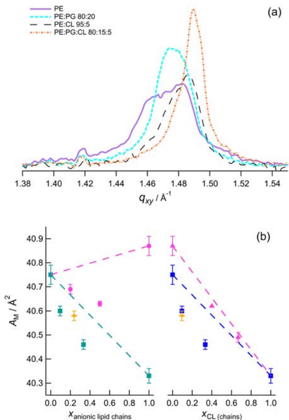
Fig. 6 (a) Comparison of the Bragg peaks derived from the images in Fig. 5. \Pi = 23 \text{ mN m}^{-1} . (b) Left: Area per molecule as a function of anionic lipid content in DMPE (pink circles PE:PG, teal triangles PE:CL). Right: Area per molecule as a function of CL content (blue circles PE:CL, pink triangles PG:CL). The orange open shapes are the values for the ternary mixture. \Pi = 40 \text{ mN m}^{-1} . The dashed lines indicate areas expected for ideal mixing.
